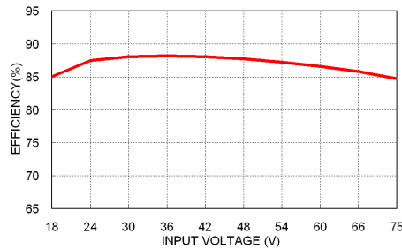
LED15-48S05W Efficiency vs. Input Voltage
