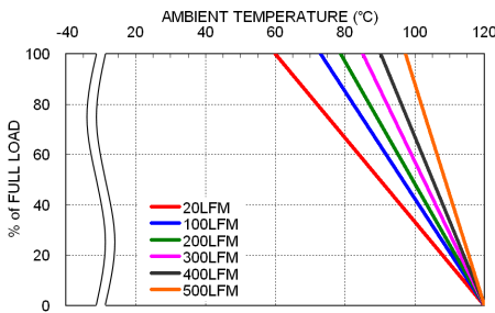
LED15-48S05W Derating Curve
