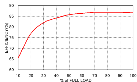
UFEC30-48S05W Efficiency vs. Output Load
