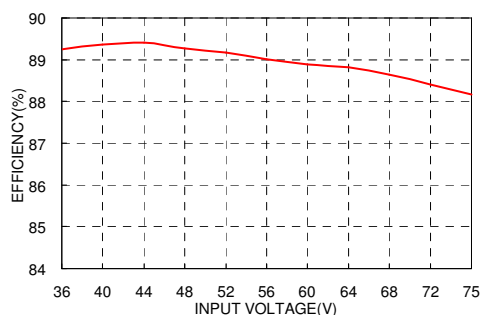
QEB125-48S05 Efficiency VS Voltage
