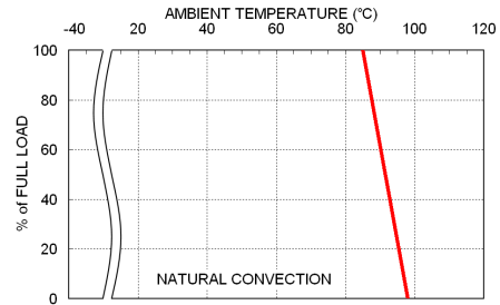
FKC03-48S05-M1 Derating Curve
