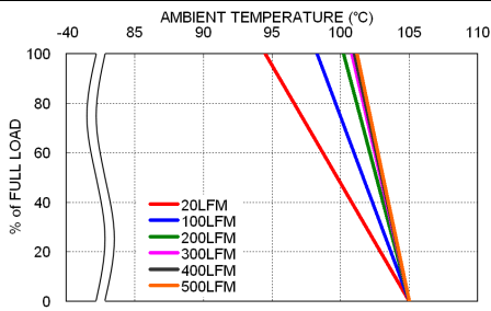
MPP03-48S05WA Derating Curve
