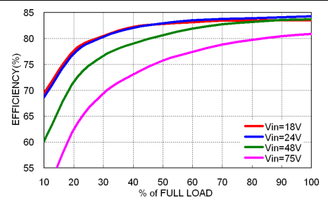
MPP03-48S05WA Efficiency vs. Output Load
