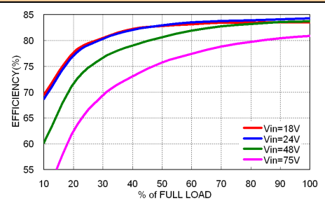
MOP03-48S05WA Efficiency vs. Output Load
