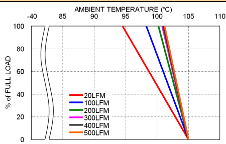
MOP03-48S05WA Derating Curve
