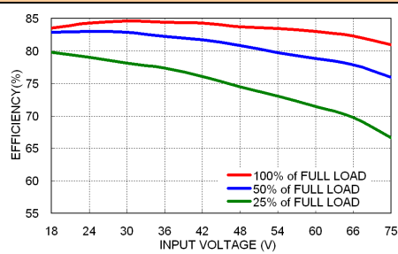
MOP03-48S05WA Efficiency vs. Input Voltage
