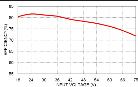
PDS02-48S05W Efficiency vs. Input Voltage
