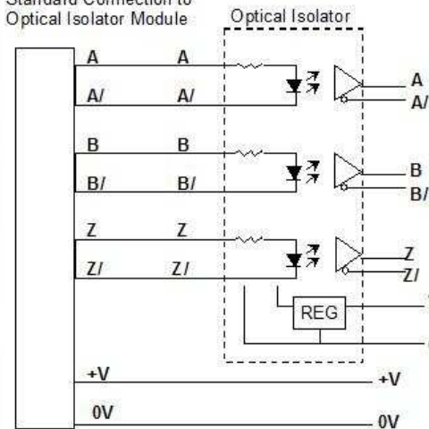
Encoder Differential Line Driver Output
