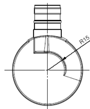
DHM5_06 connection G6R (radial M23), flange 9500/003* mounted on the body
