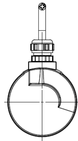
DHM5_06 connection G6R (radial M23), flange 9500/003* mounted on the body
