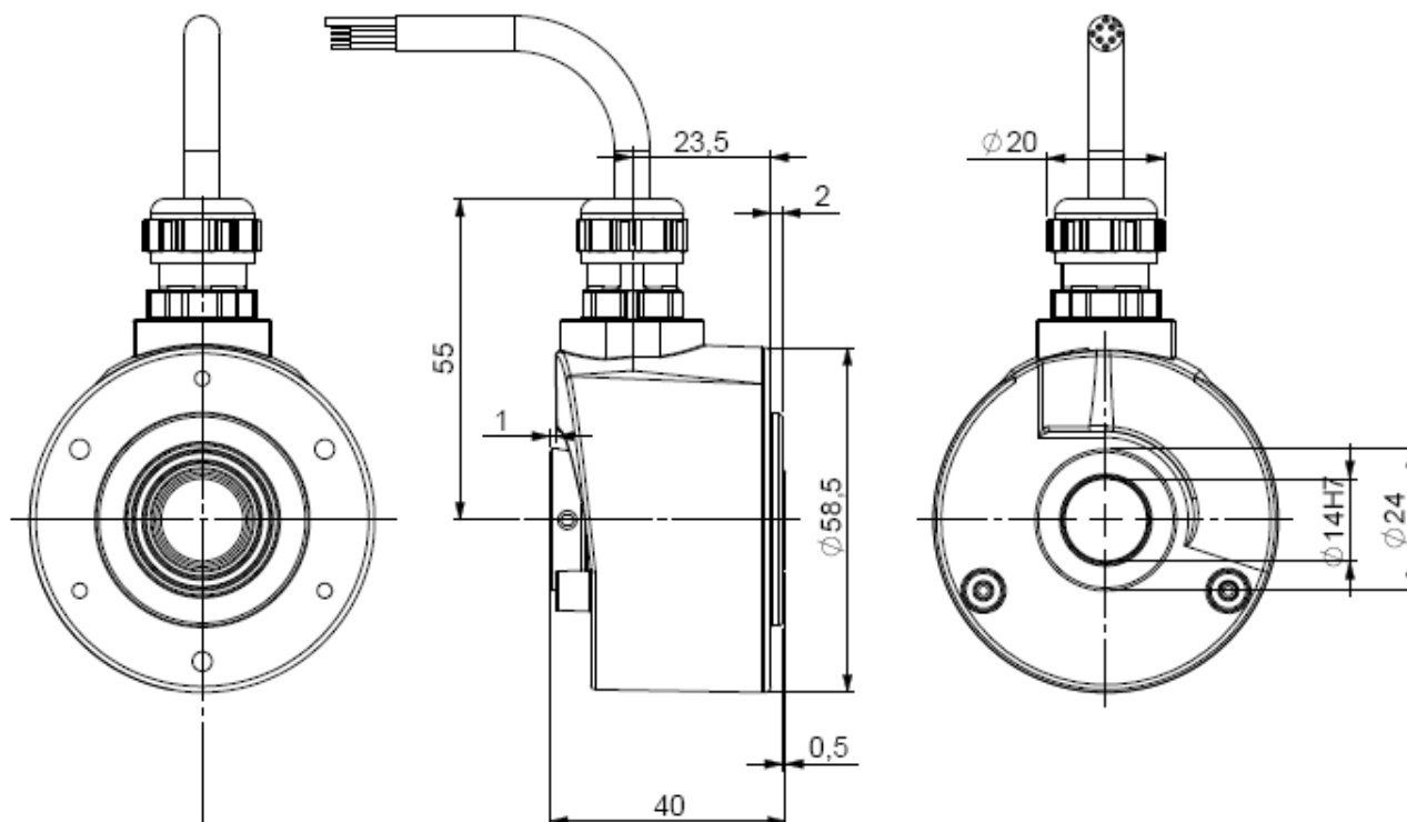
IBO5_14 with connection G3R (radial cable)
