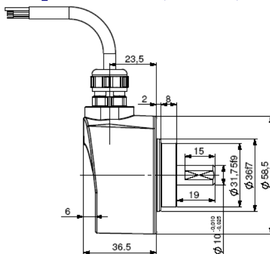
IBM5_10 connection G3R(radial cable)
