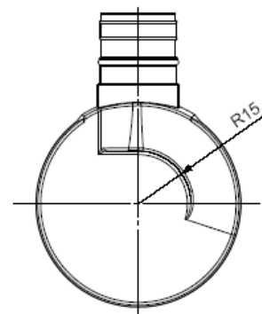
IBM5_06 connection G6R(radial M23), flange 9500/003 mounted onto the body
