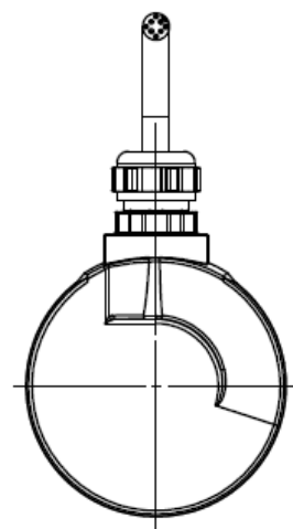
IBM5_06 connection G6R(radial M23), flange 9500/003 mounted onto the body
