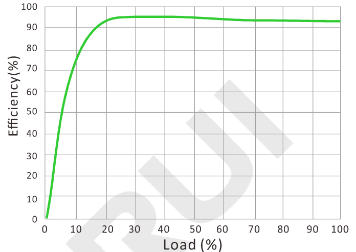
EFFICIENCY CURVE
