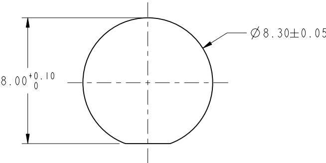
SCALE 4.200 RECOMMENDED MOUNTING HOLE DIMENSIONS
