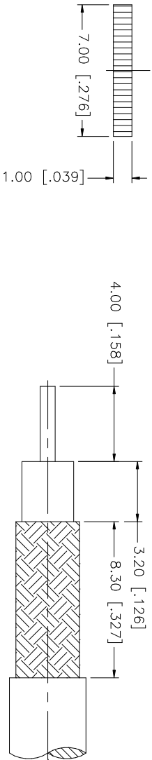
RECOMMENDED CABLE STRIPPING DIM'S
