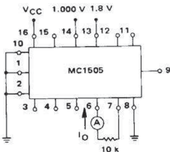
FIGURE 4 – I_O MEASUREMENT
