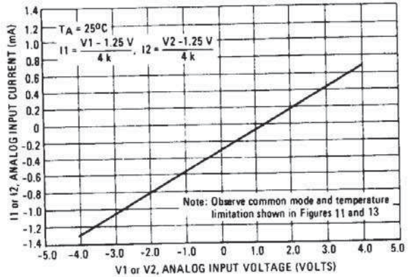
FIGURE 14 – INPUT CURRENT versus INPUT VOLTAGE
