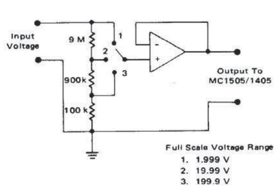
FIGURE 24 – DVM VOLTAGE RANGING
