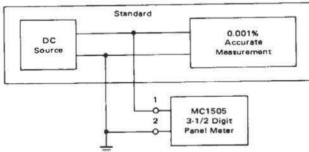
FIGURE 10 - CALIBRATION SET-UP
