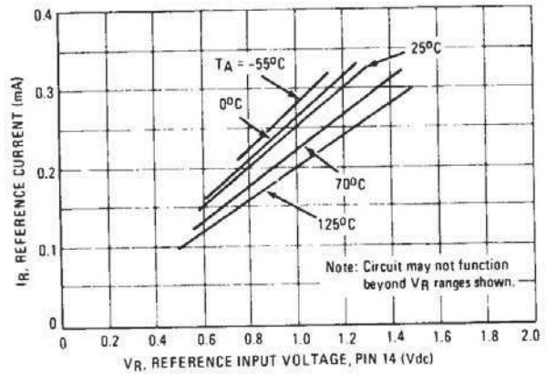
FIGURE 16 – REFERENCE CURRENT versus REFERENCE INPUT VOLTAGE
