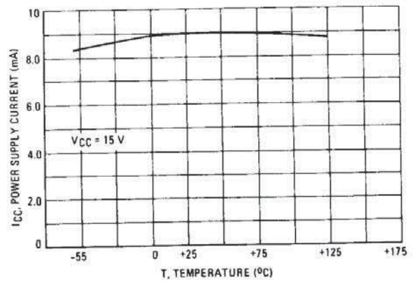
FIGURE 18 – TYPICAL POWER SUPPLY CURRENT versus TEMPERATURE
