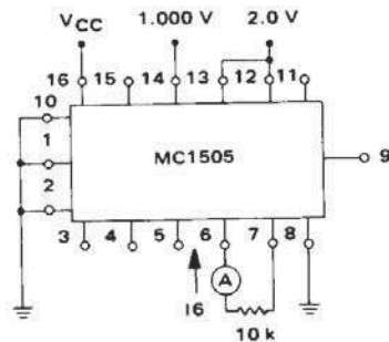
FIGURE 5 – I6 MEASUREMENT
