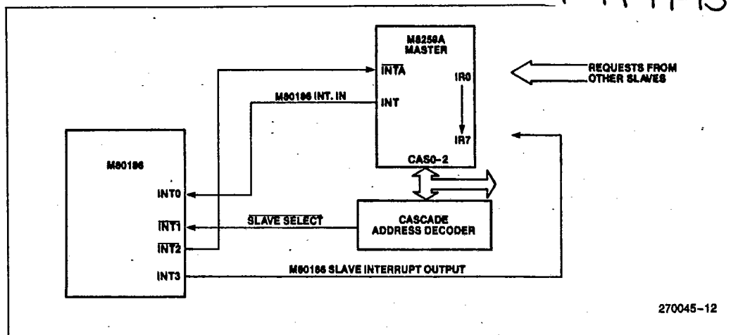
Figure 32. MiRMXTM 86 Interrupt Controller Interconnection
