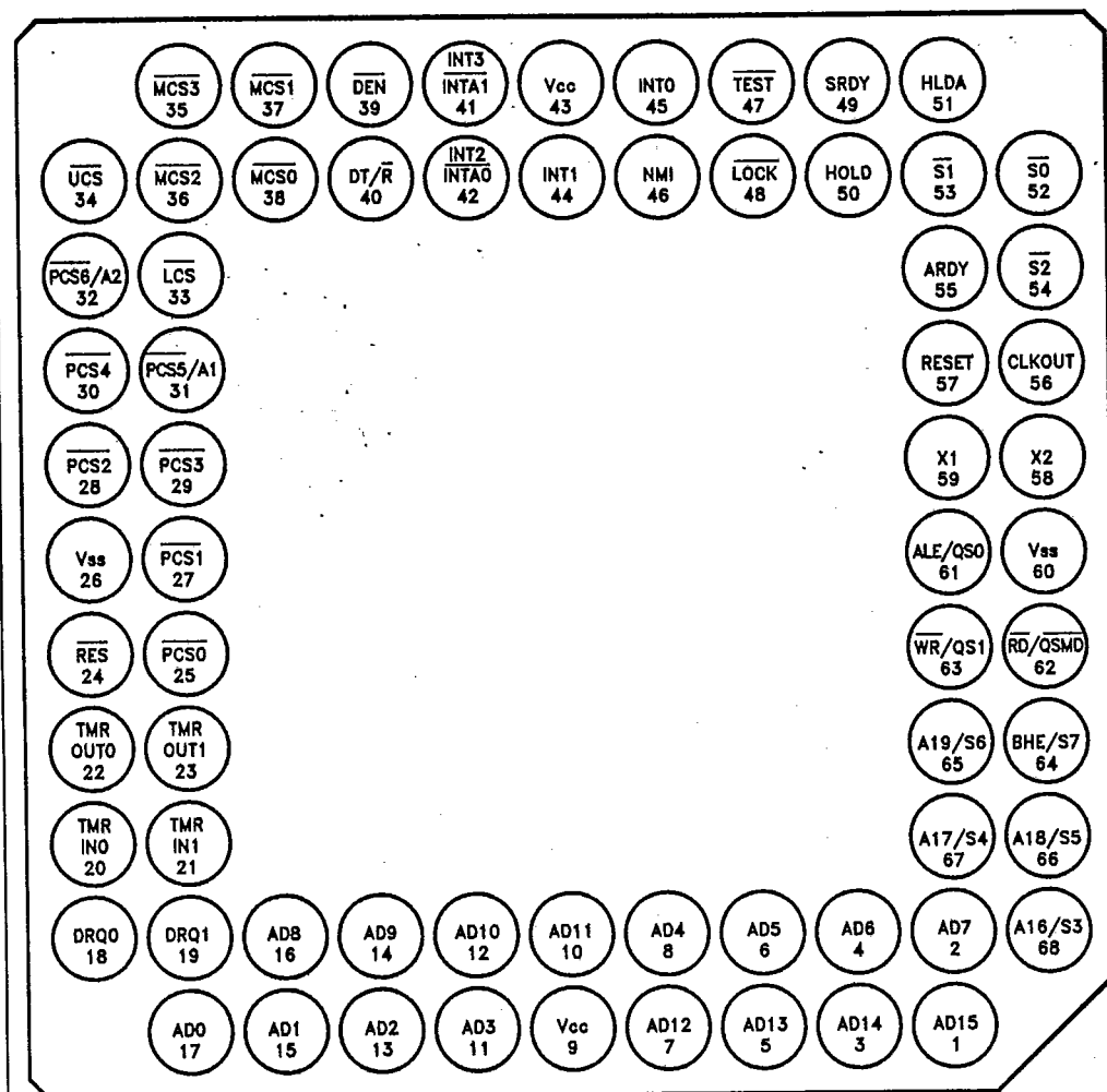
Figure 42. Pin Grid Array
