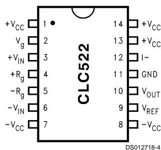
Pinout DIP & SOIC
