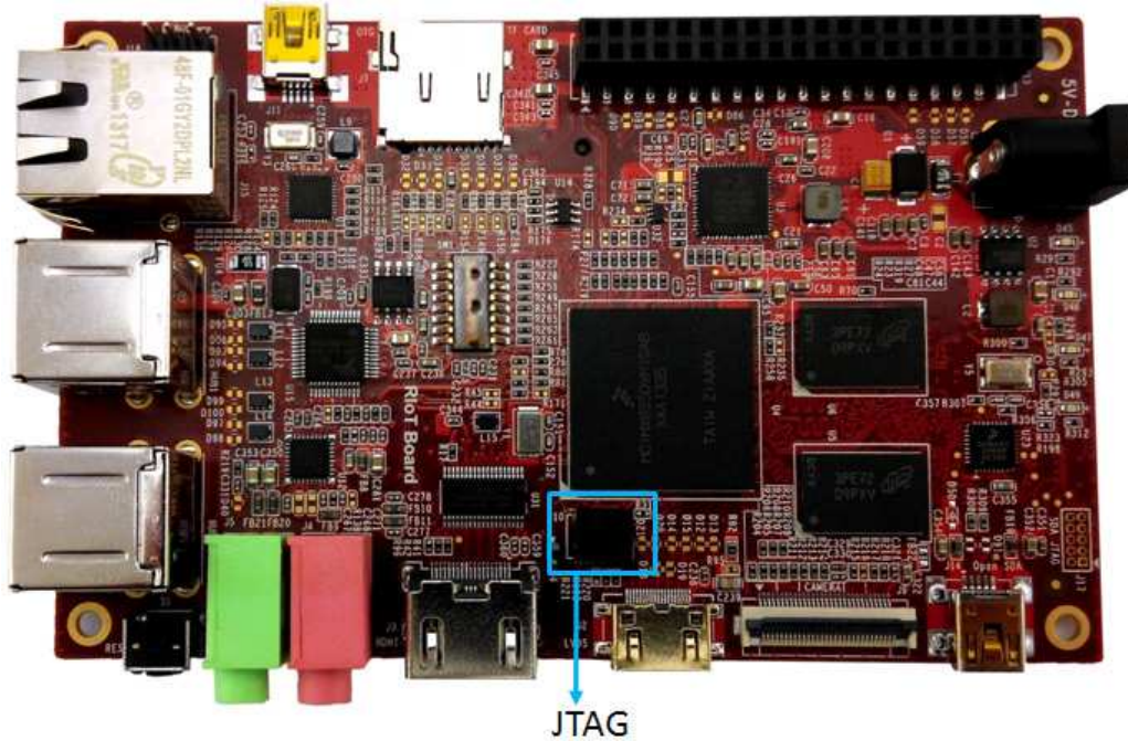
Figure 2-11 JTAG Interface
