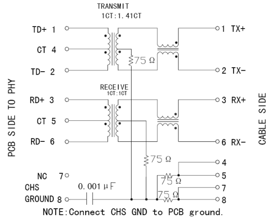
MOXIE MOX-RJ45TD-018
