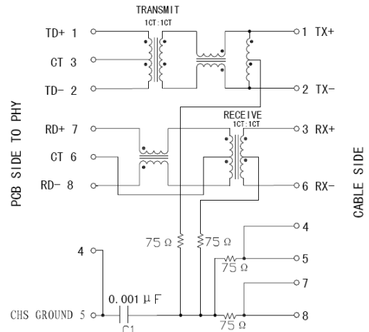
MOXIE MOX-RJ45TD-026
