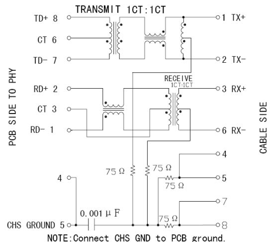
MOXIE MOX-RJ45TD-035
