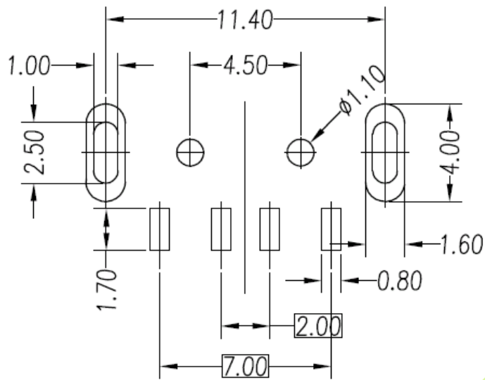
RECOMMAND PCB LAYOUT TOLERANCE \pm 0.05
