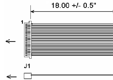
DISCRETE-WIRE CABLE SECTION
