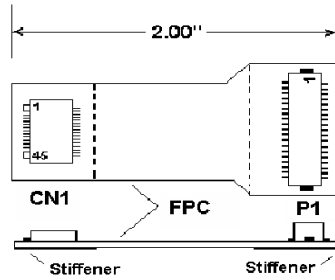
FPC ADAPTER SECTION
