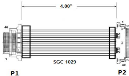
SMALL GAUGE COAX JUMPER
