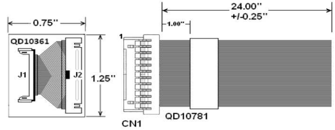
PCB ADAPTER DISCRETE WIRE FLYING LEAD ASSY
