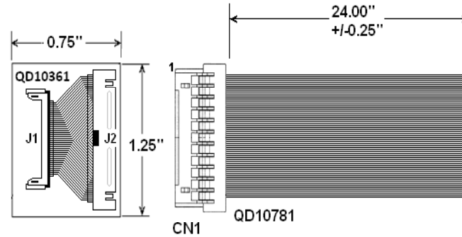
PCB ADAPTER
