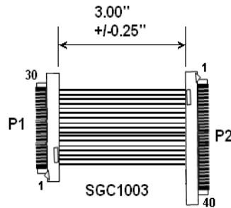
SMALL GAUGE COAX JUMPER
