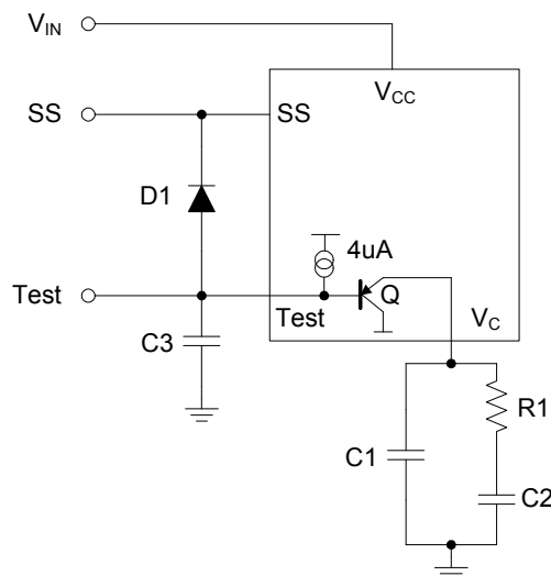
Figure 31. Soft-Start
