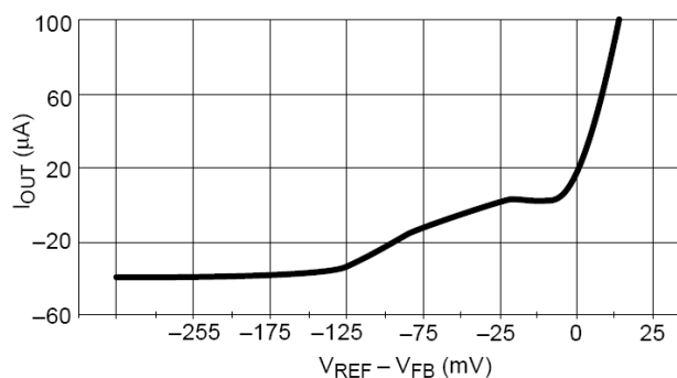
Figure 18. Error Amplifier Iout vs. Vfb
