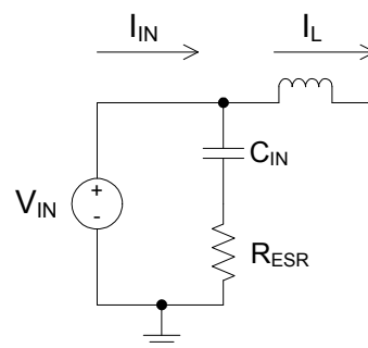
Figure 26. Boost Circuit Effective Input Filter
