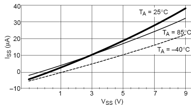
Figure 14. Iss vs Vss
