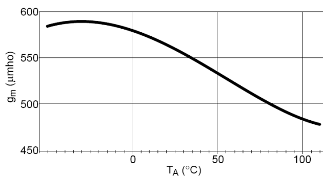
Figure 16. Error Amplifier Transconductance vs. Temperature
