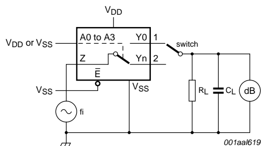
Fig 15. Test circuit for measuring isolation (OFF-state)
