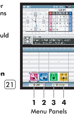
Settings Panel
