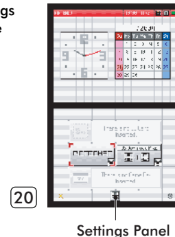
Settings Panel
