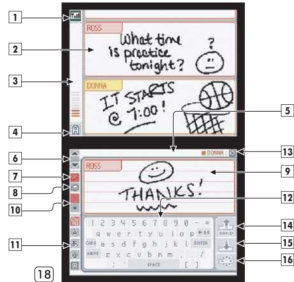
PictoChat Screen
