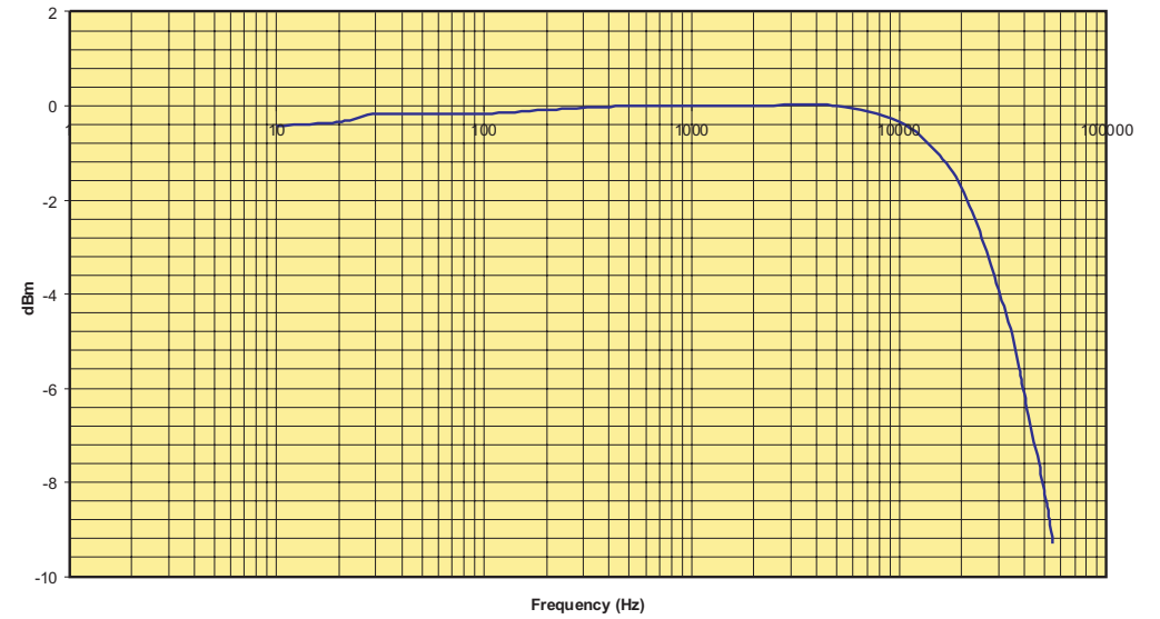
Frequency response: source: 0dBm, load: 1628 ohms, windings in series
