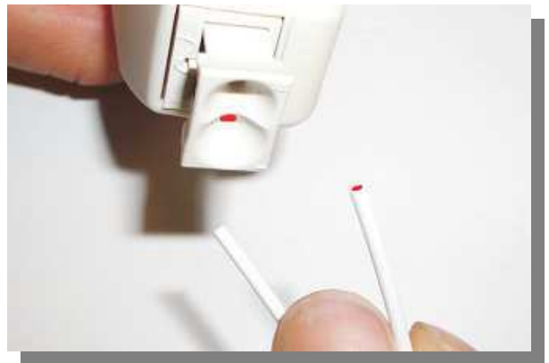
FIGURE 2 Split the POF strands.
