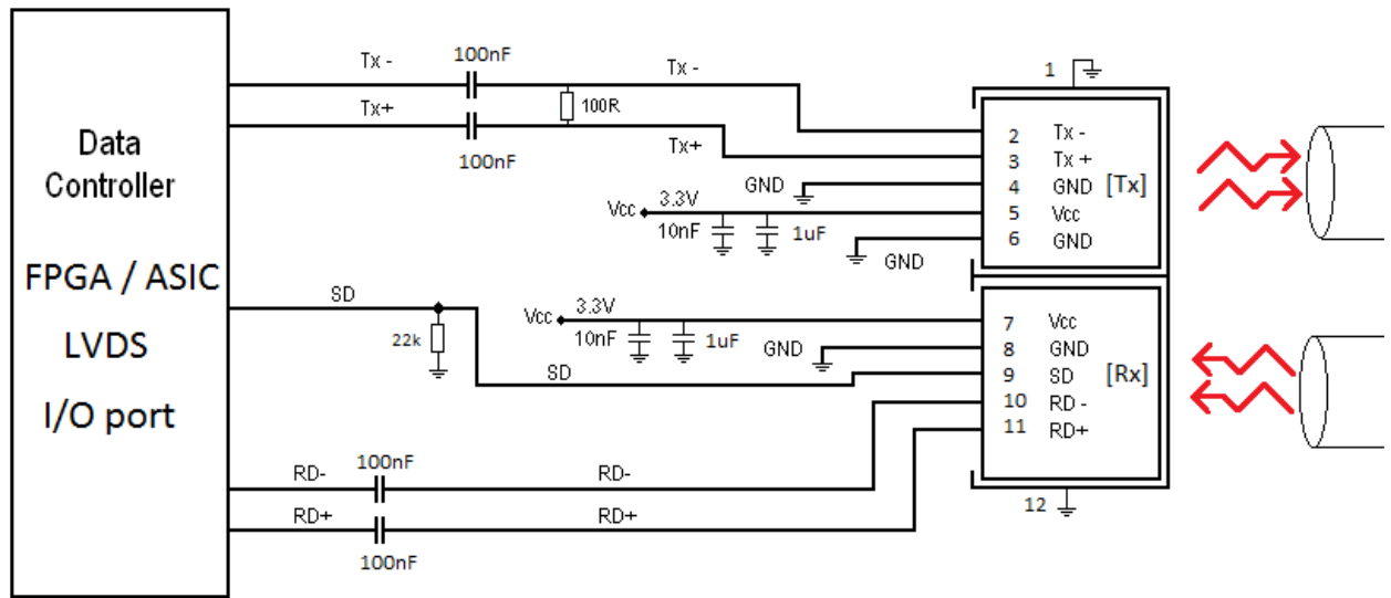
FIGURE 12 Interface circuit schematic to AC couple to a PHY, FPGA or ASIC IC where the IC will not accept a common mode voltage of 1.2V
