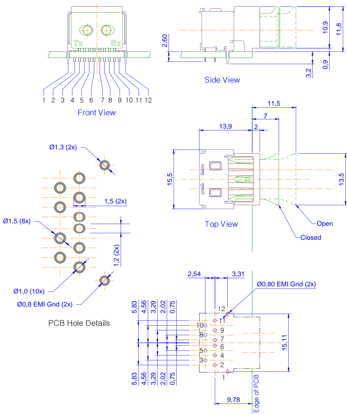
FIGURE 13 Mechanical dimensions of the OptoLock connector and PCB footprint, which is a top view. General dimensional tolerance is \pm 0.2\text{mm} .
