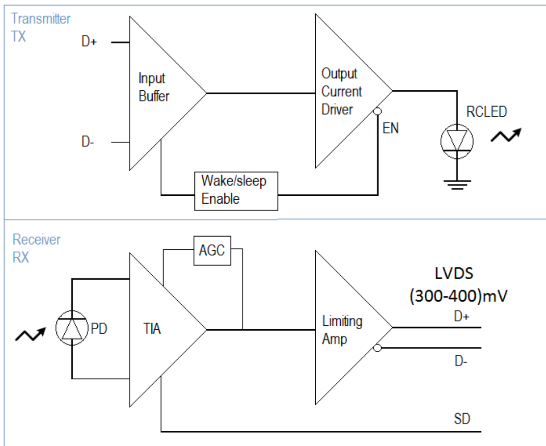
FIGURE 10 OptoLock transceiver electronic block diagram
