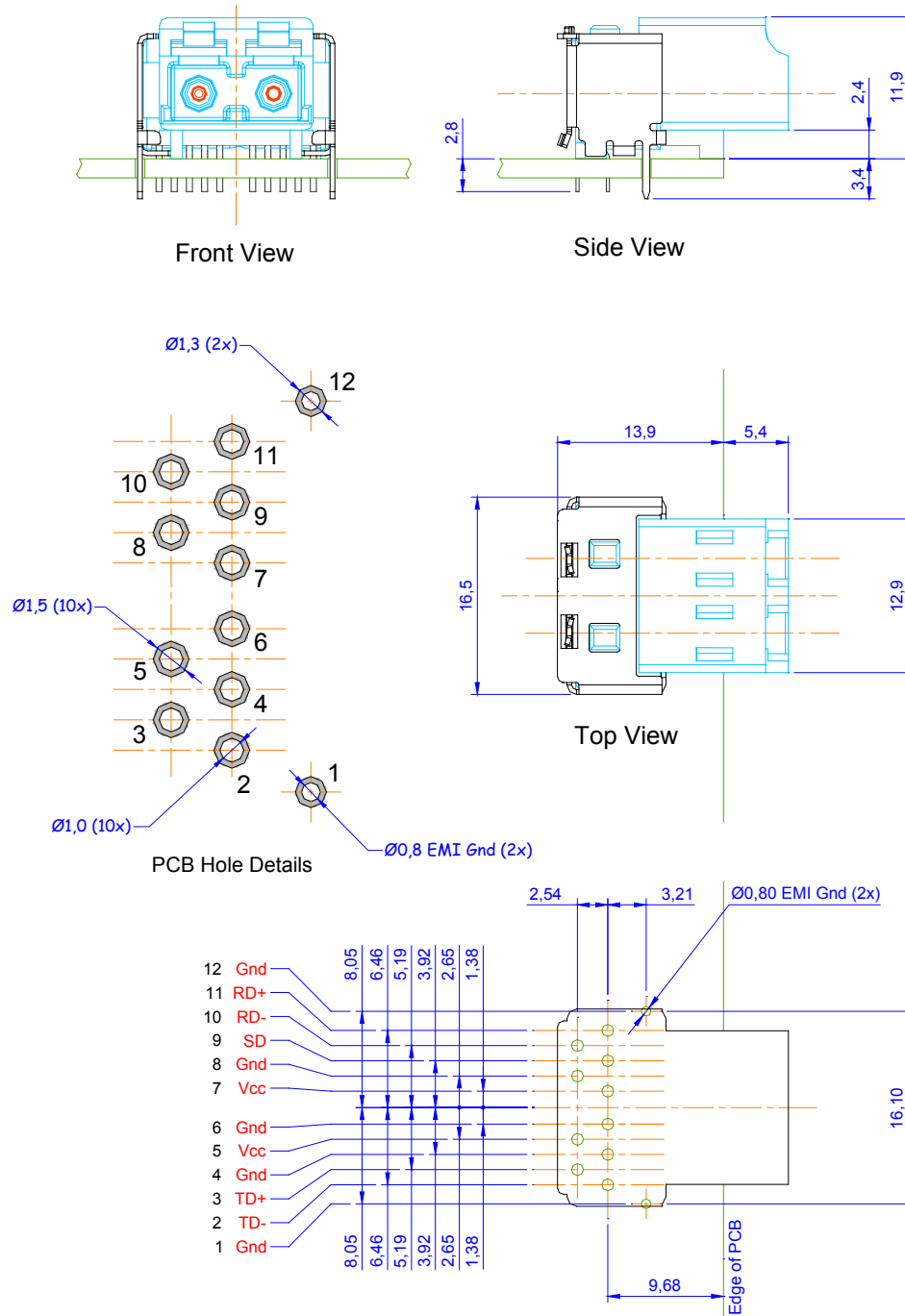
FIGURE 5 Mechanical dimensions of the LC connector and PCB footprint, which is a top view. General dimensional tolerance is \pm 0.2 mm.
