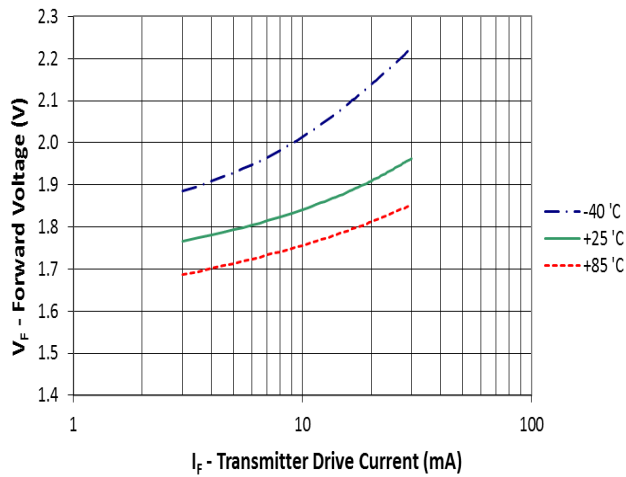
FIGURE 2 Typical forward voltage (VF) vs. drive current (IF,DC).
