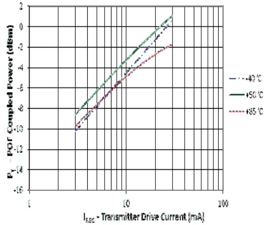
FIGURE 3 Typical normalized optical power vs. drive current.
