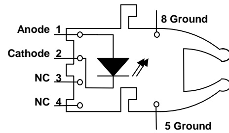
FIGURE 4 RedLink low current transmitter PCB footprint, top-view.
