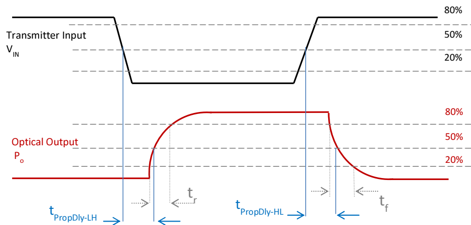
FIGURE 1 Transmitter propagation delay and rise/fall time definitions.
