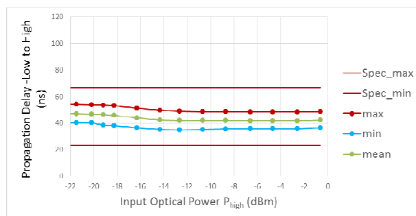
FIGURE 14: Propagation Delay for Output Low to High Transitions.
