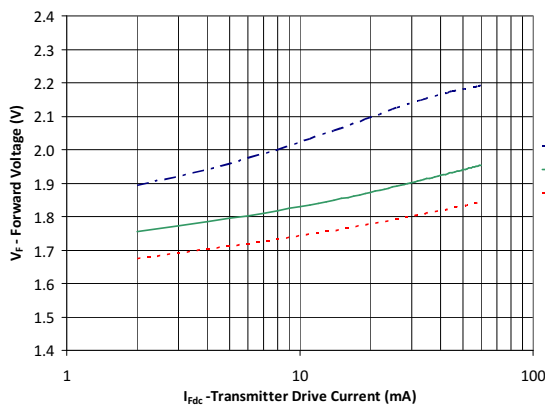
FIGURE 2 Typical forward voltage vs. drive current.
