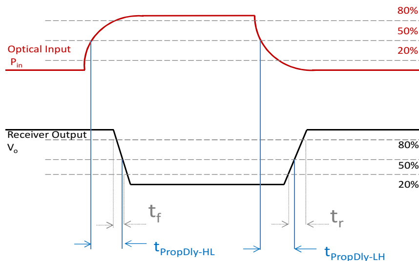
FIGURE 9 Receiver Propagation Delay and rise/fall time definitions.
