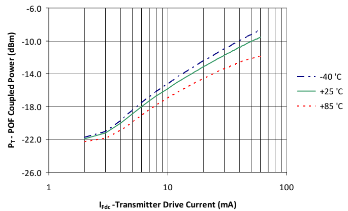
FIGURE 3 Typical optical output power vs. drive current.
