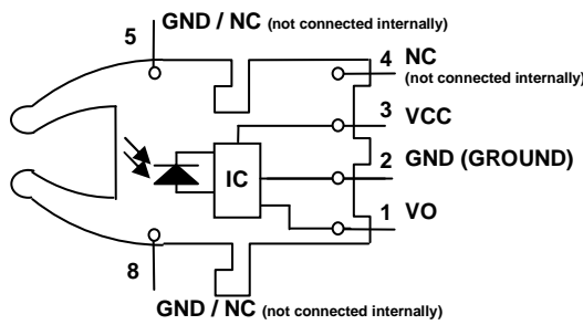
FIGURE 18 Receiver pin numbering.
