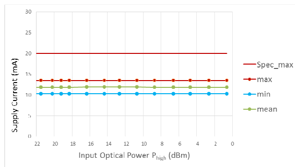
FIGURE 12: Supply current over all operating conditions.
