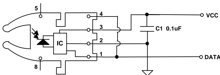
FIGURE 19 RedLink receiver interface circuit.
