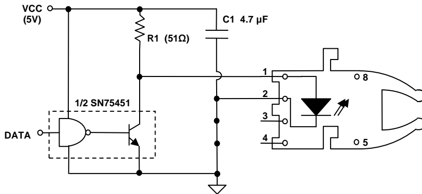
FIGURE 7 Non-inverting application circuit for the FT05MHNR; for temperature range 0°C to +70°C, use SN75451B as the driver IC, for temperature range -40°C to +85°C, use SN55451B. I F,ON = 60 mA nominal at +25°C.
