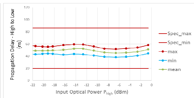
FIGURE 15: Propagation Delay for Output High to Low Transitions.
