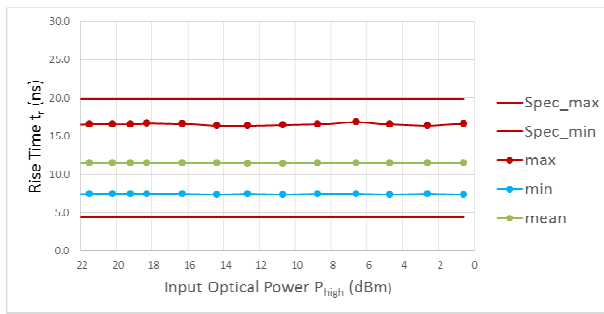
FIGURE 16: Receiver output rise time t_r over all operating conditions.
