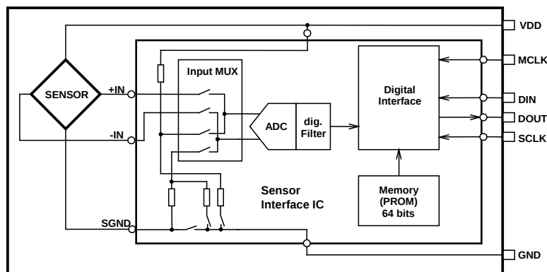
Fig. 1: Block diagram MS5535C
