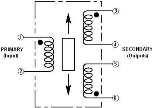
Connect 4 to 5 for differential output
