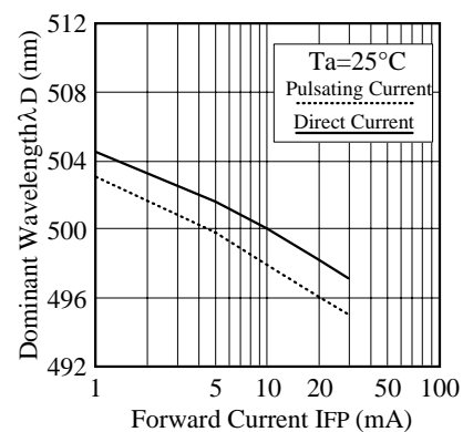
■ Forward Current vs. Dominant Wavelength * * Pulsating Current
