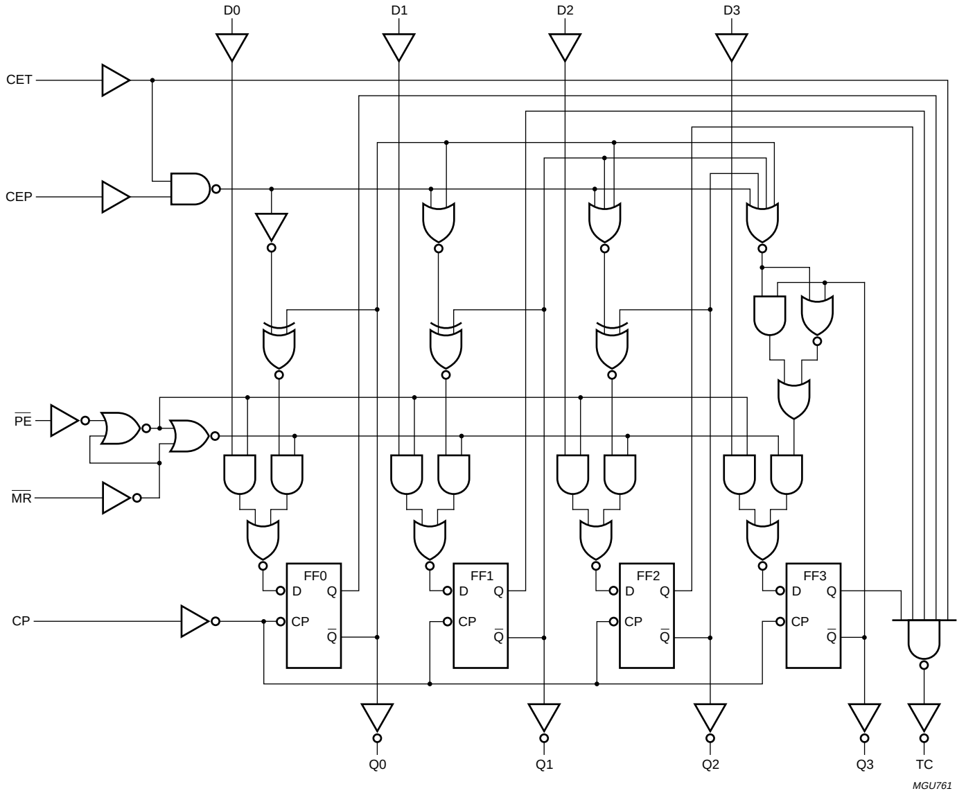
Fig.8 Logic diagram.
