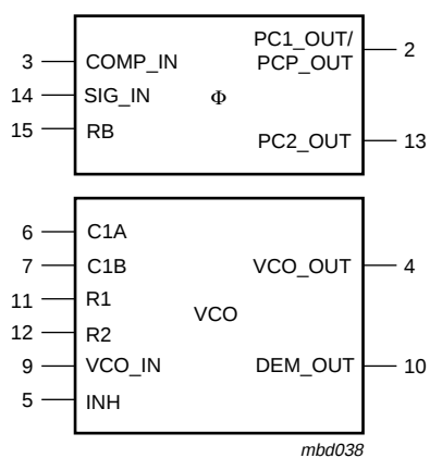
Fig 2. Logic symbol
