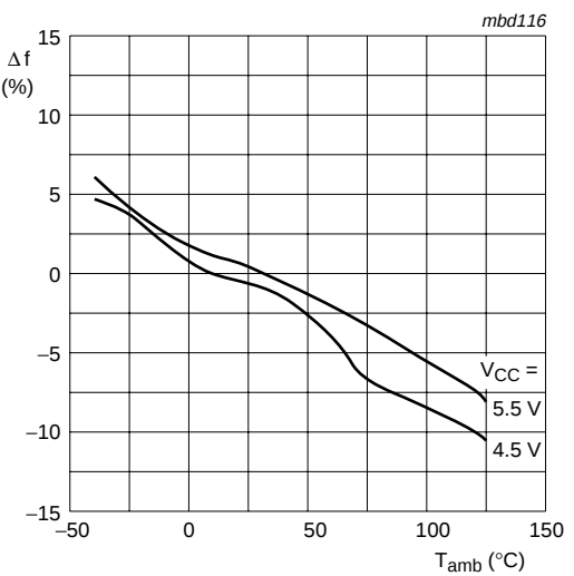
Fig 20. Frequency stability of the VCO as a function of ambient temperature with supply voltage as a parameter
