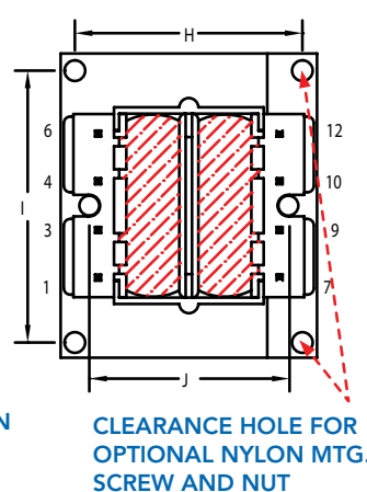
BOTTOM VIEW
