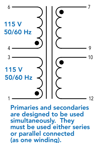
SCHEMATIC
