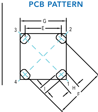
RECOMMENDED PCB PATTERN
