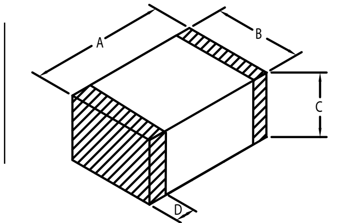
ISOMETRIC VIEW
