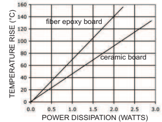
POWER DERATING
