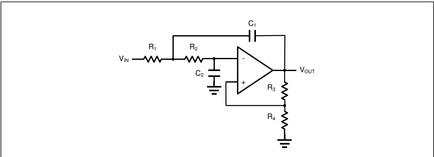
Figure 9. Sallen-Key 2nd Order Active Low-Pass Filter
