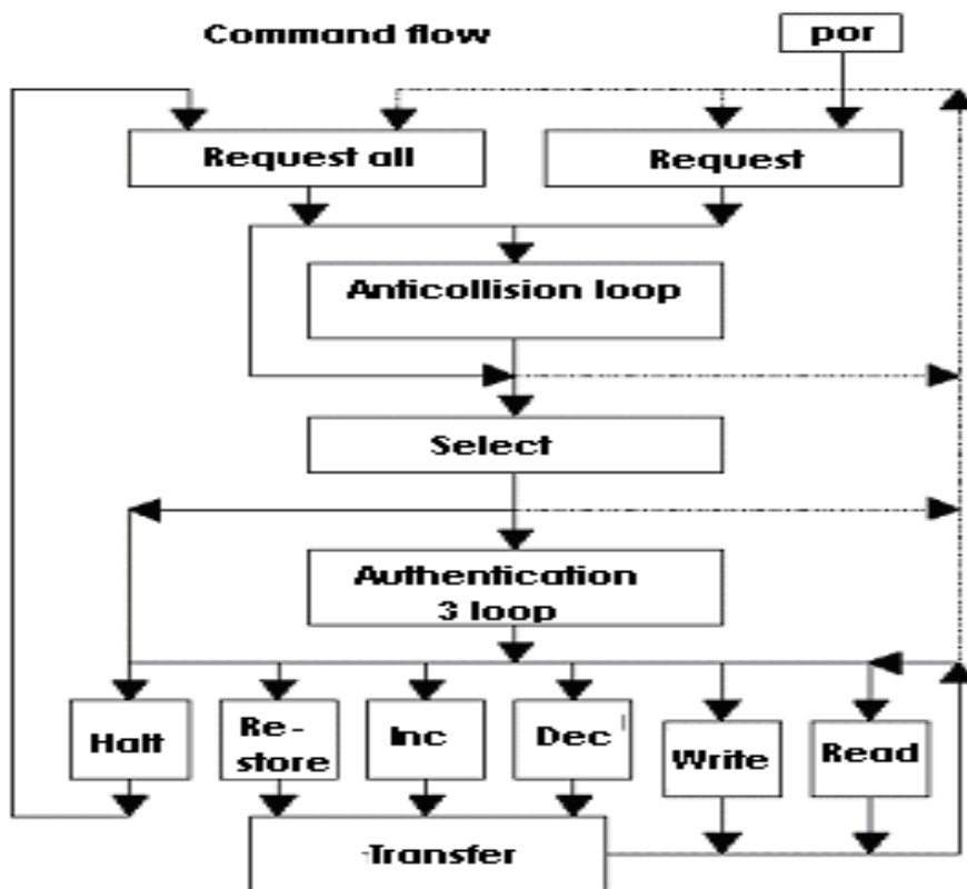
Fig. 2 Communication Flow
