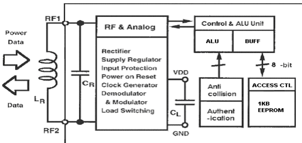
Fig. 1 Block Diagram
