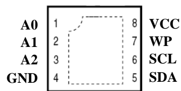
8-Lead UDFN
