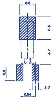
RECOMMENDED LAND PATTERN
