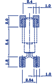
RECOMMENDED LAND PATTERN
