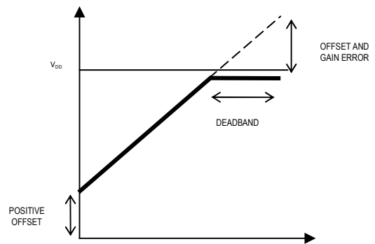
Figure 5. Effect of Gain Error and Positive Offset
