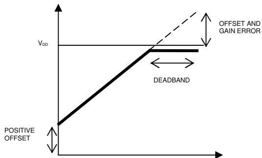
Figure 7. Effect of Gain Error and Positive Offset
