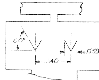
DETAIL OF TABS SHOWN IN BLANK FORM.
