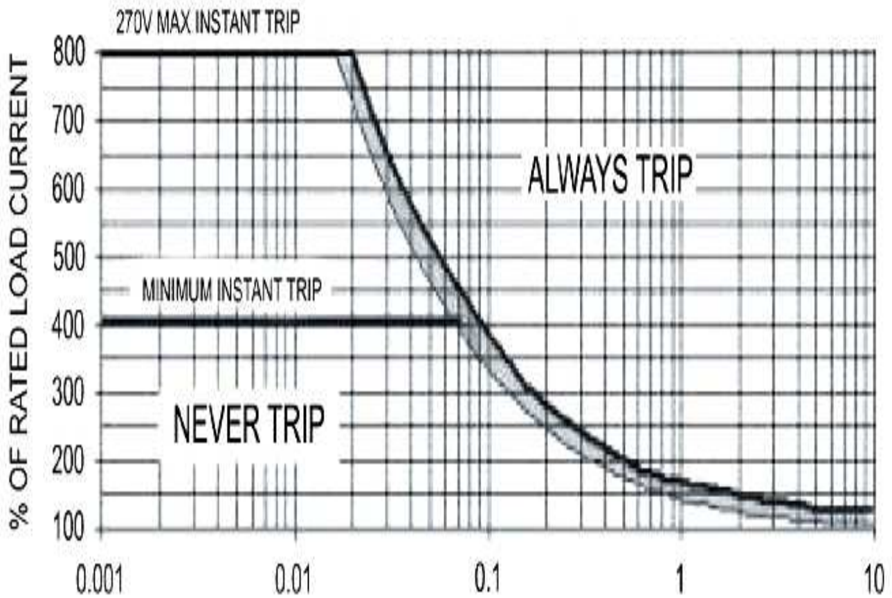
Figure 1 - Trip Curve
