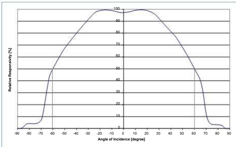
Figure 1 Typical Field of View Curve (Sensor Orientation A)
