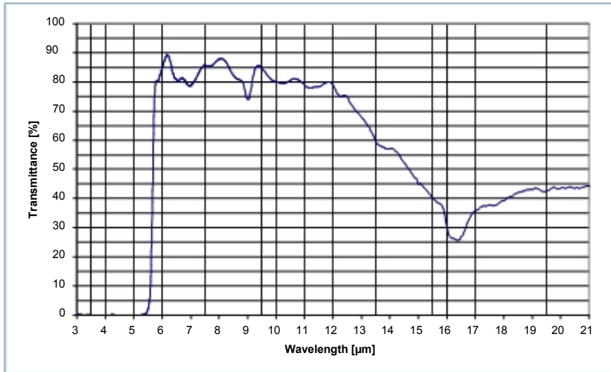
Figure 3 Transmission Curve for Excelitas Standard Filter
